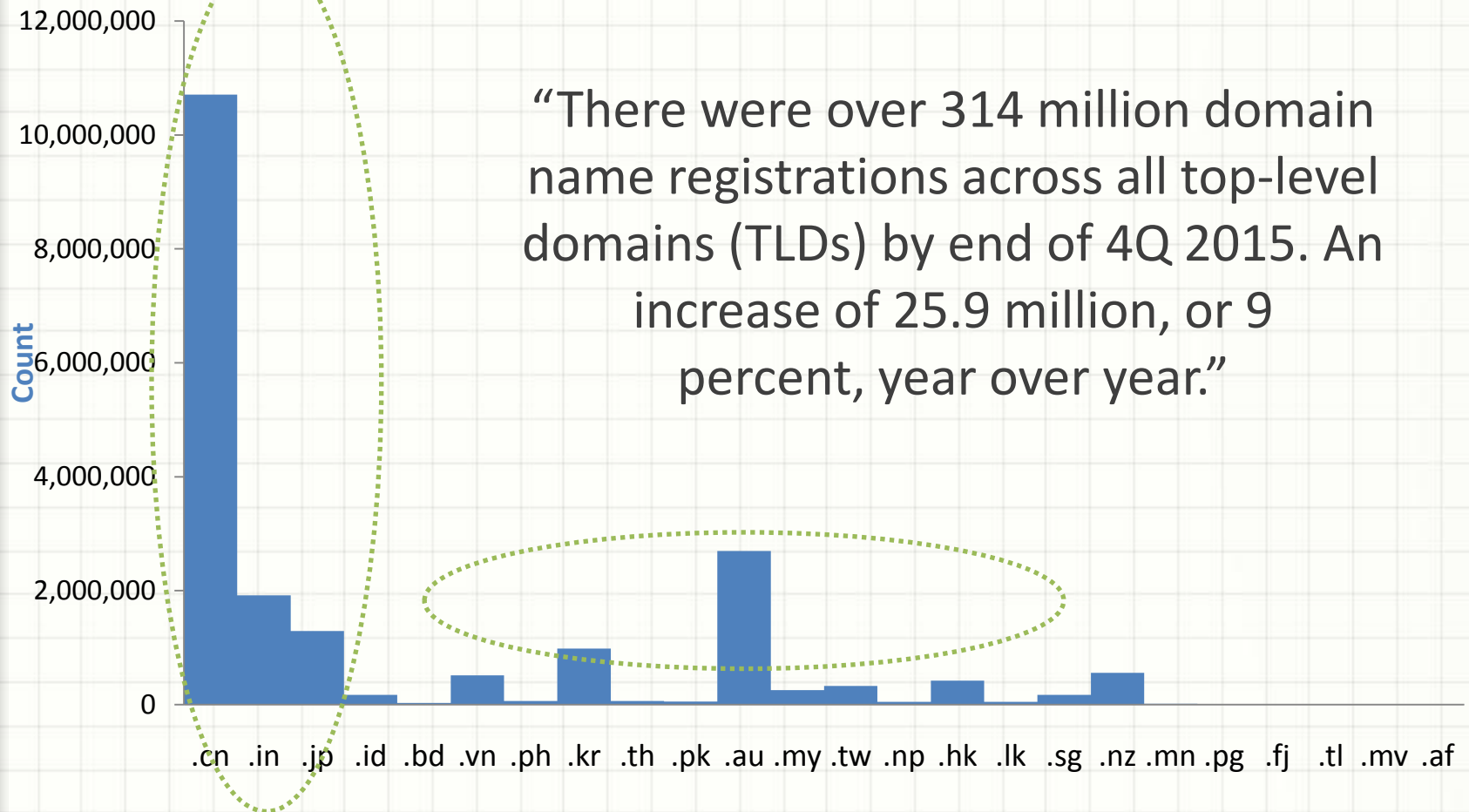
ccTLD Count
